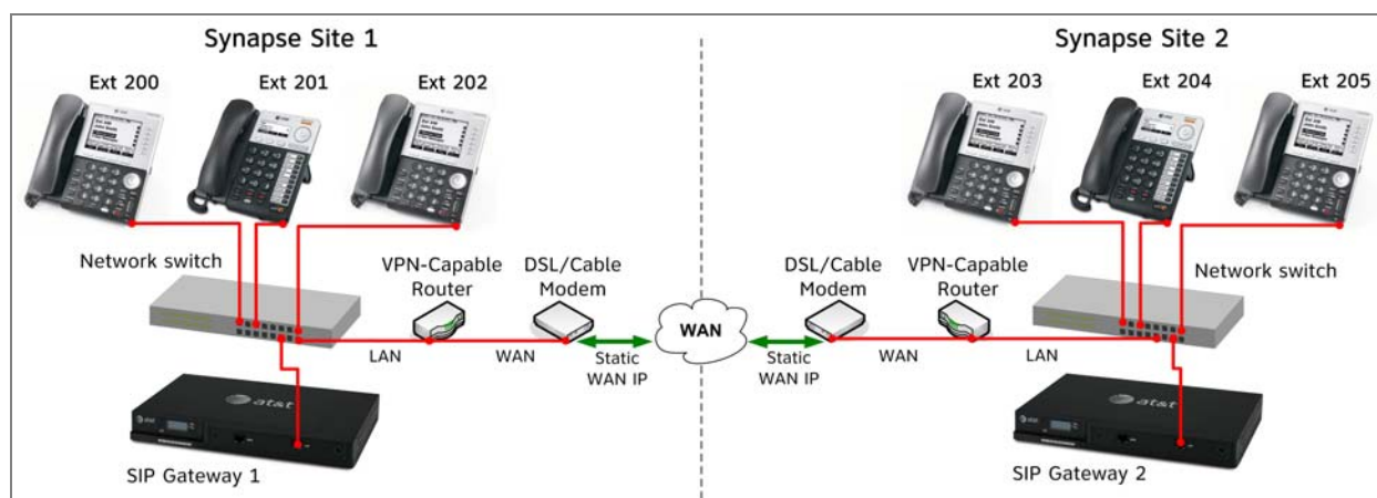
Figure 3. Example of Remote Site Installation
