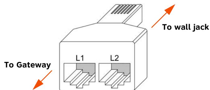
Figure 4. Two-line Adapter
